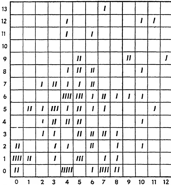
FIG. XII Scatter diagram. Correlation of approximately +0.3.
